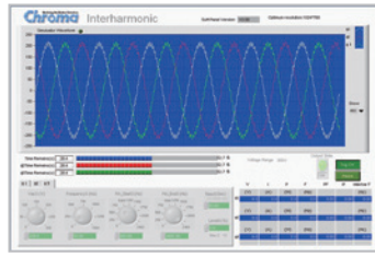
Inter-harmonic Test
