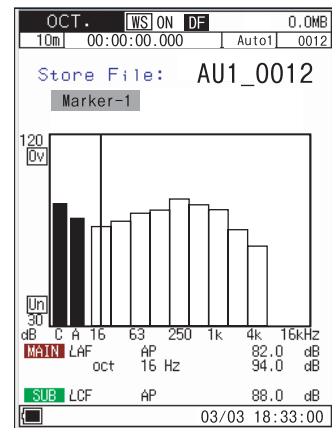
Recall screen, analyzer mode
