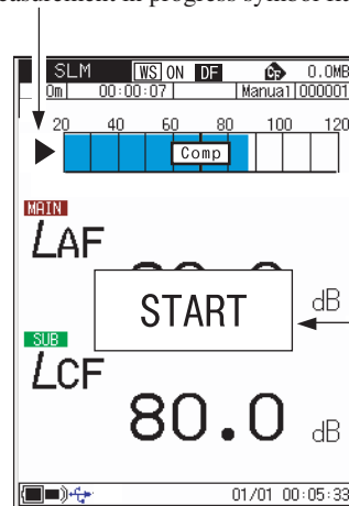
Measurement screen
