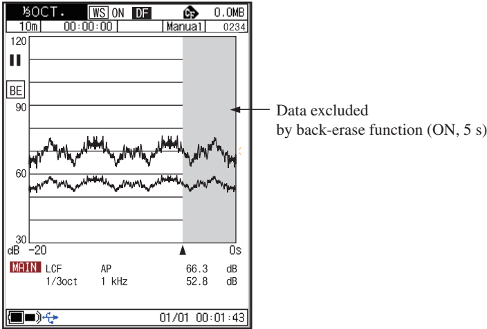
Time-Level screen
