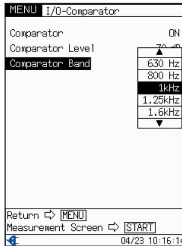
I/O - Comparator menu screen
