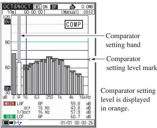
Analyzer mode indication
